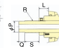
PU203~PU205 (Drawbar connection)
