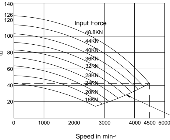
Gripping Characteristic Graph For BB210A8
