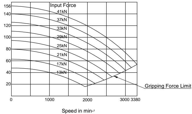
Gripping Characteristic Graph For N-12A6
